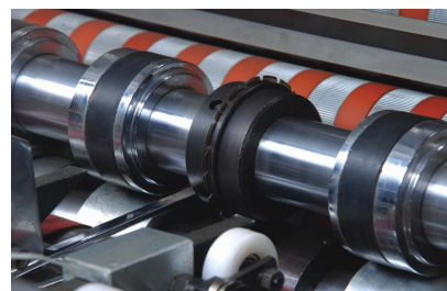
Perforation/slitting/creasing
